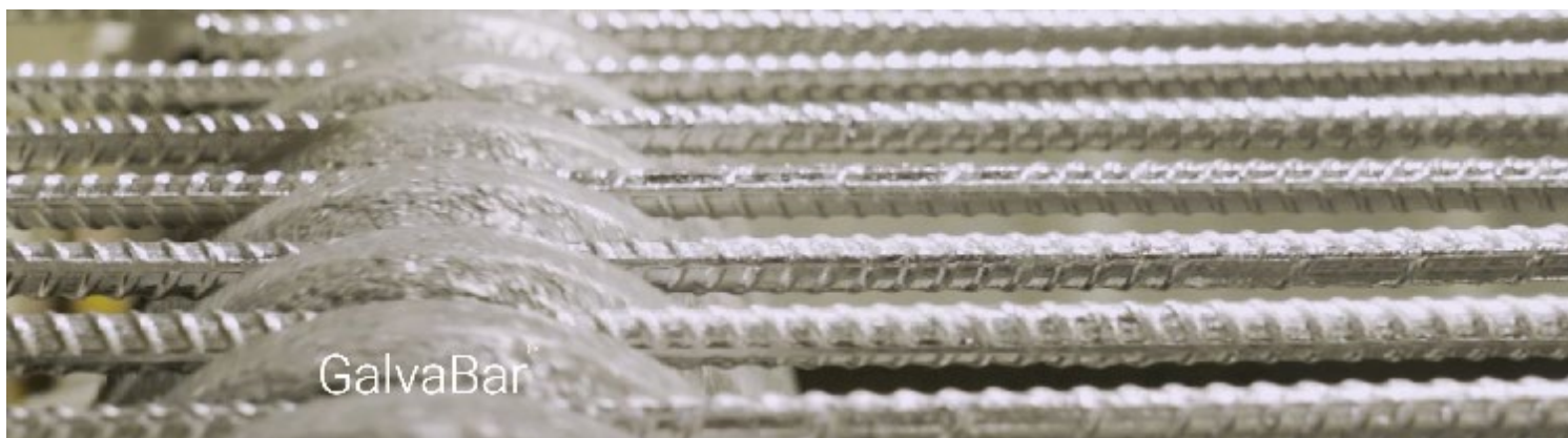
Image of GalvaBar® in the molten bath from CMC's website.
