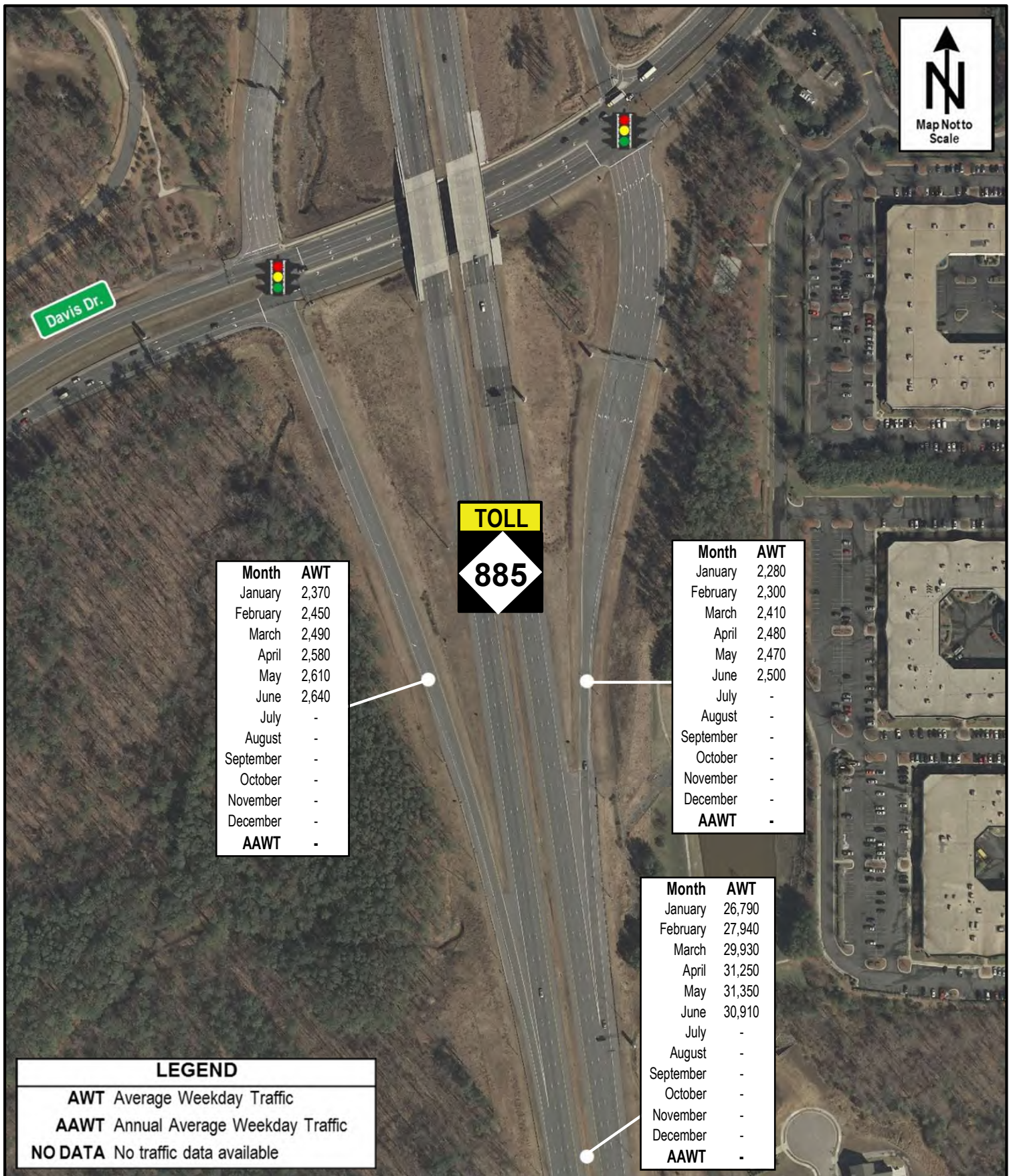
NC-885 at Davis Dr. Interchange 2026 Average Weekday Traffic
