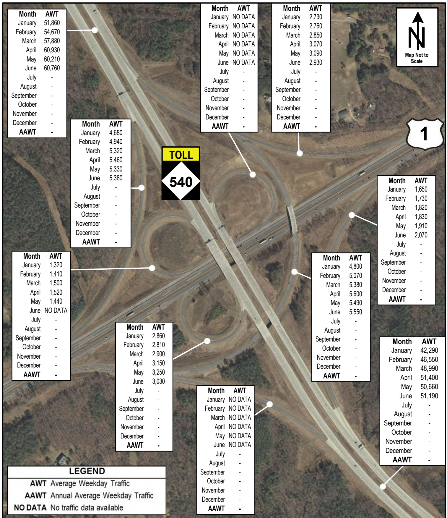
NC-540 at US-1 Interchange 2026 Average Weekday Traffic
