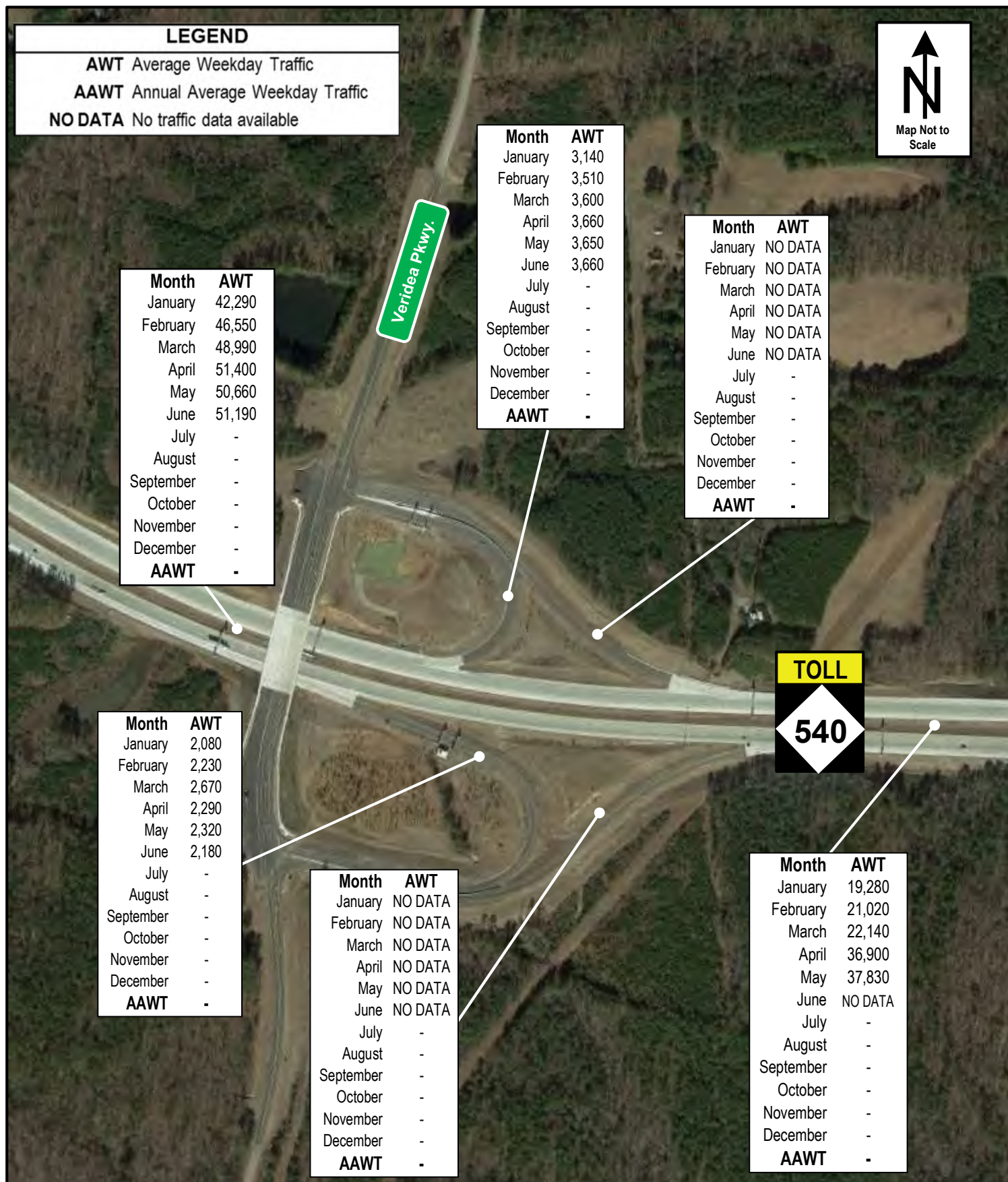
NC-540 at Veridea Pkwy. Interchange 2026 Average Weekday Traffic
