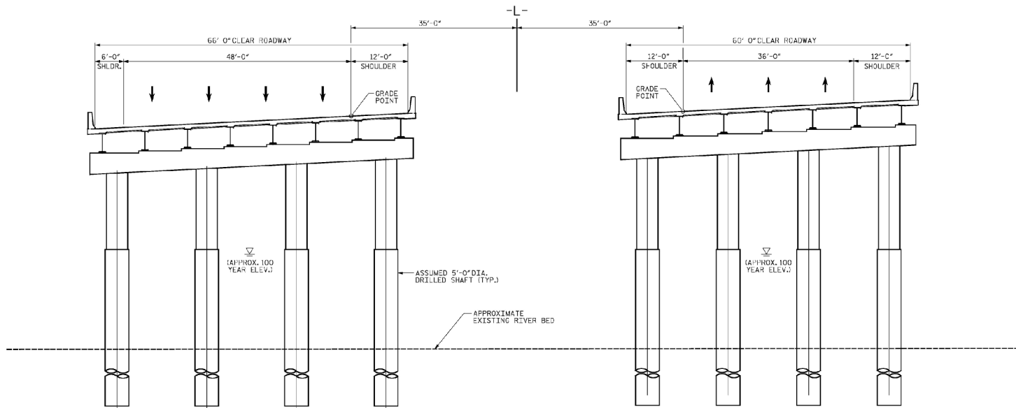
SECTION A-A (at Bent's in Neuse River)
