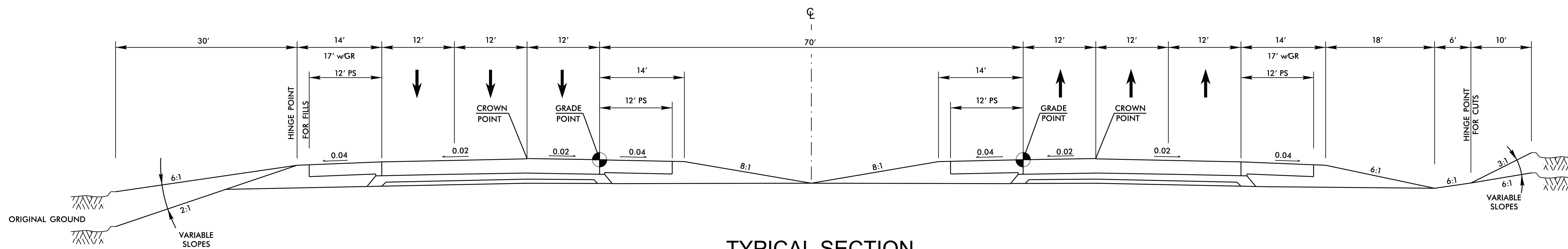
TYPICAL SECTION -L- NC 540
