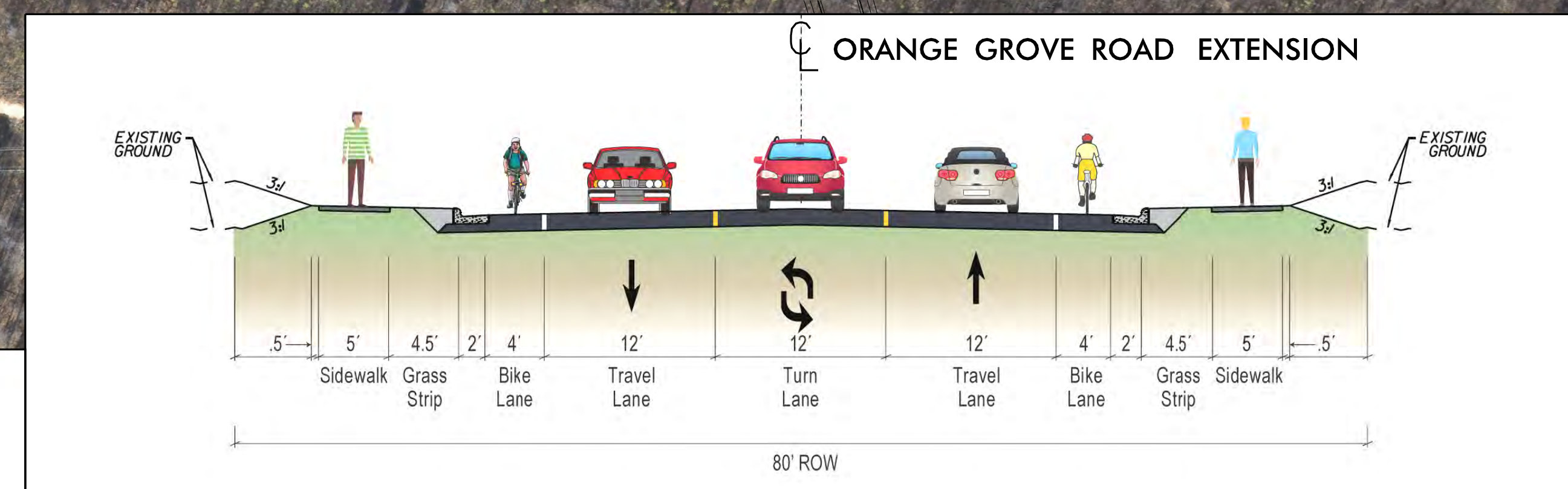
ROADWAY TYPICAL SECTION ***BIKE AND PEDESTRIAN ACCOMMODATIONS SHOWN ARE PRELIMINARY AND SUBJECT TO CHANGE PENDING COORDINATION WITH LOCAL MUNICIPALITIES
