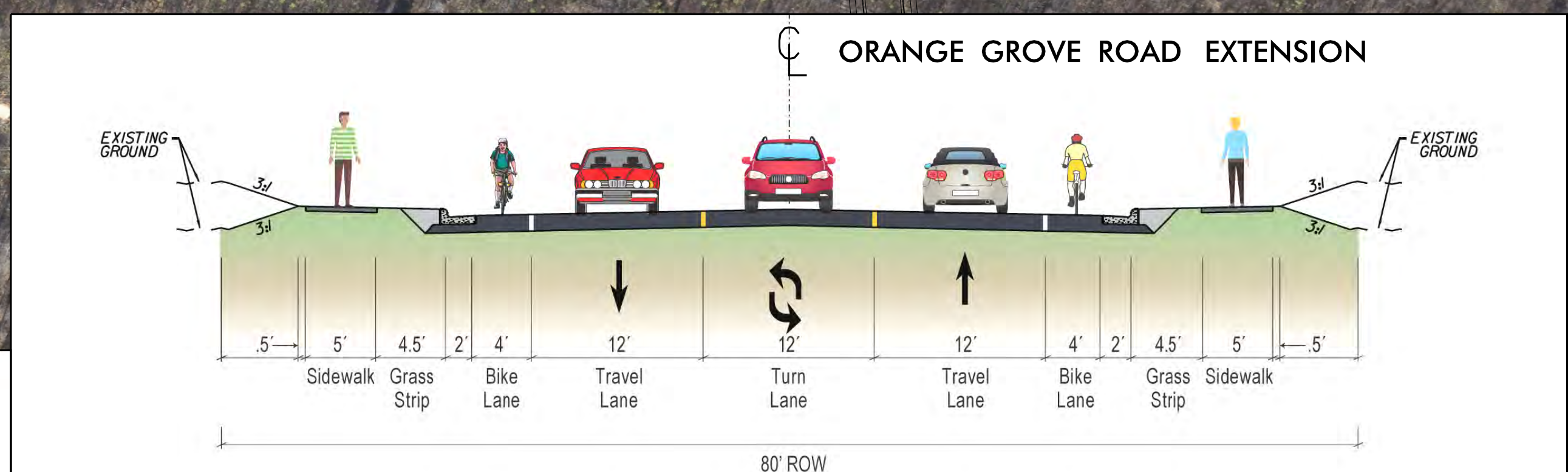
ROADWAY TYPICAL SECTION
