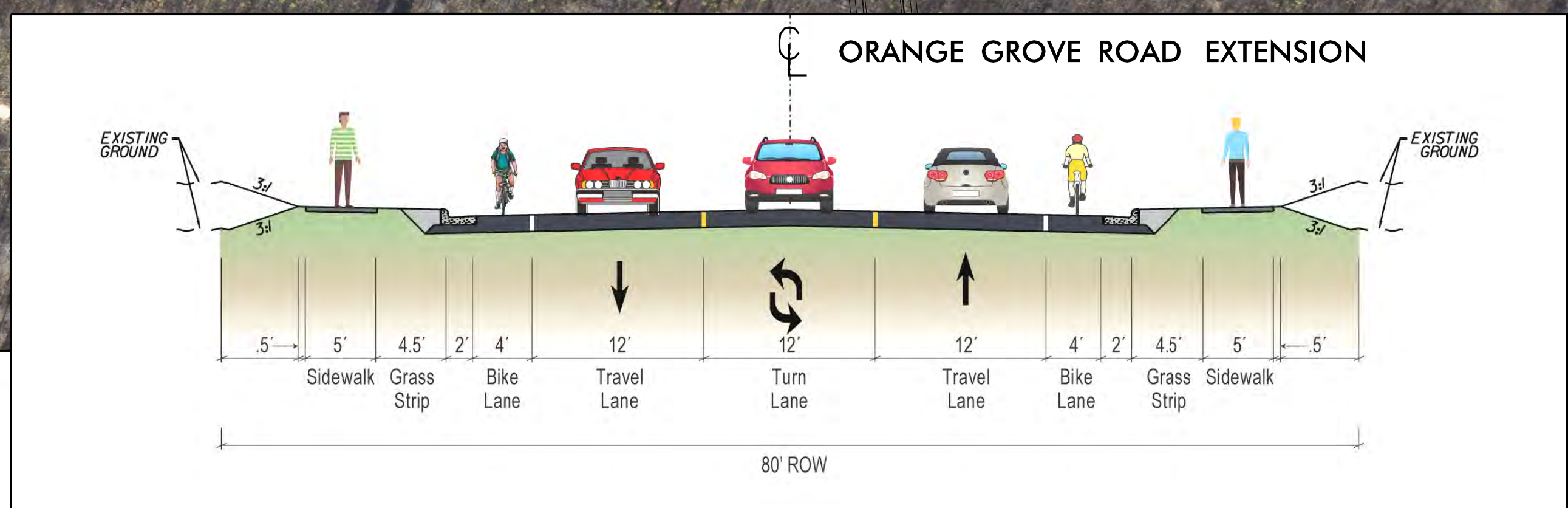
ROADWAY TYPICAL SECTION
