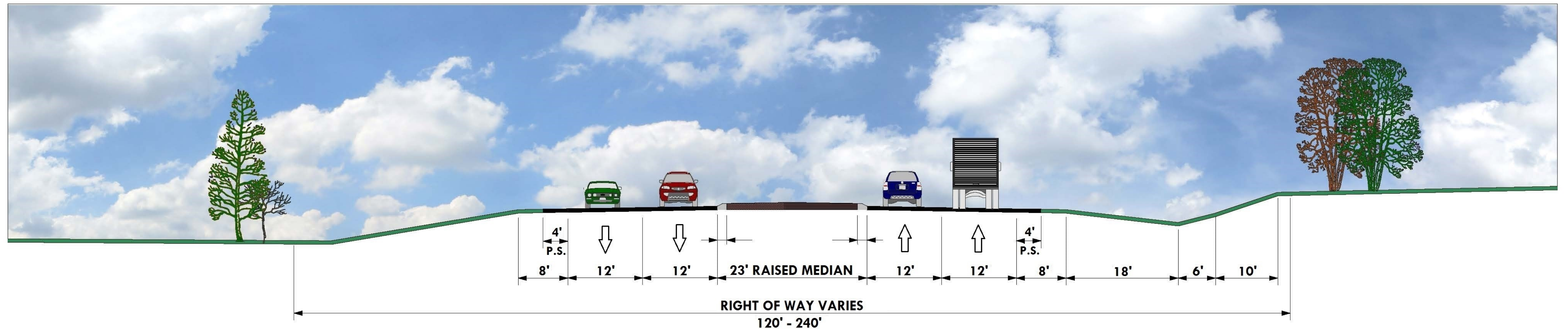
4 LANE DIVIDED (23' RAISED MEDIAN) WITH PAVED SHOULDERS POSTED SPEED 35 - 55 MPH
