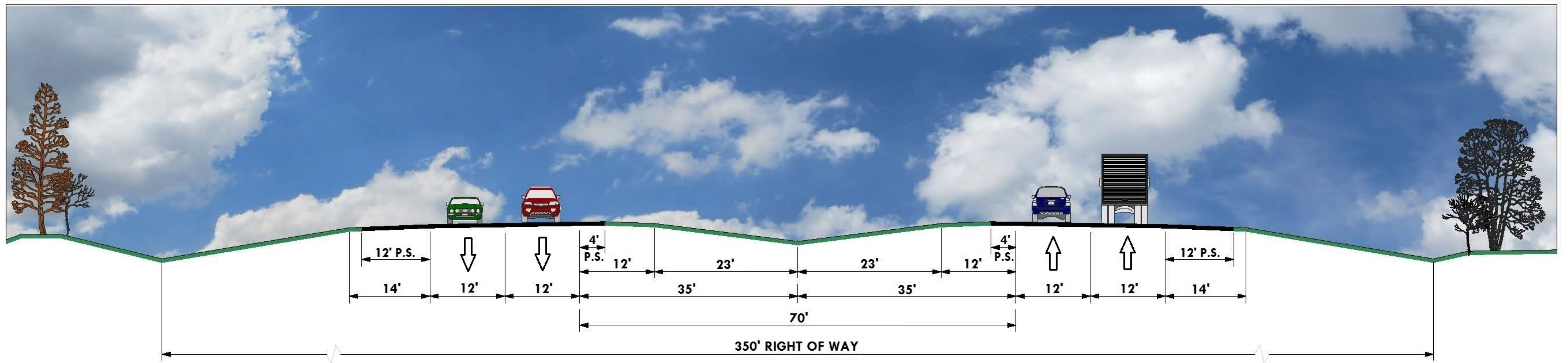
4 LANE DIVIDED (46' GRASS MEDIAN) WITH PAVED SHOULDERS POSTED SPEED 65 MPH
