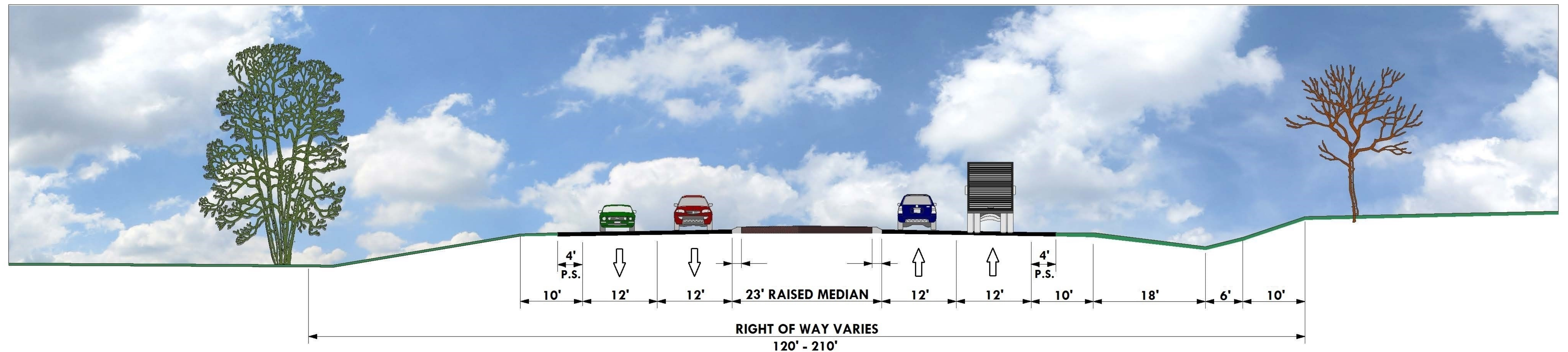
4 LANE DIVIDED (23' RAISED MEDIAN) WITH PAVED SHOULDERS POSTED SPEED LIMIT 35 - 55 MPH
